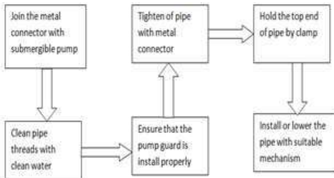
Fig. 1: Steps in installation procedureBlock diagram is shown above giving the details activities to be
