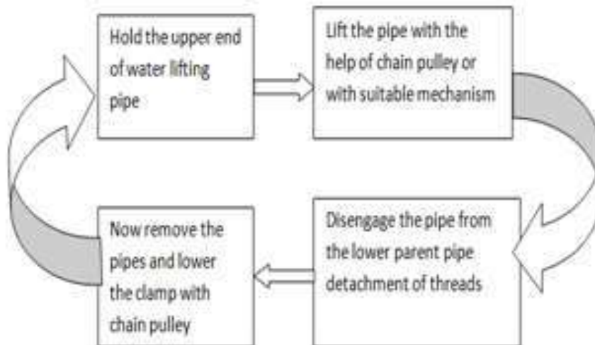
Fig. 3: Steps in lifting Process
